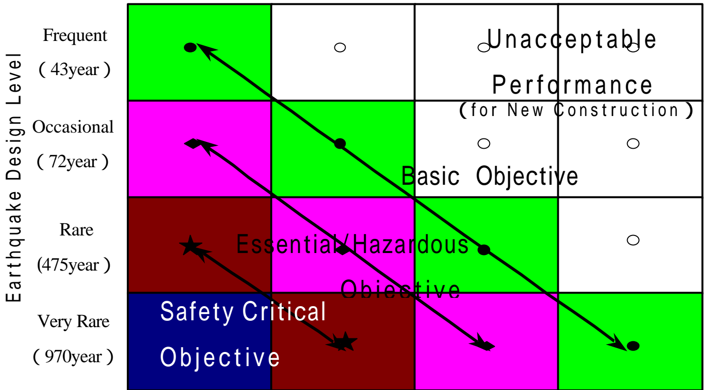
Fig: Recommended Performance Objectives for Buildings
