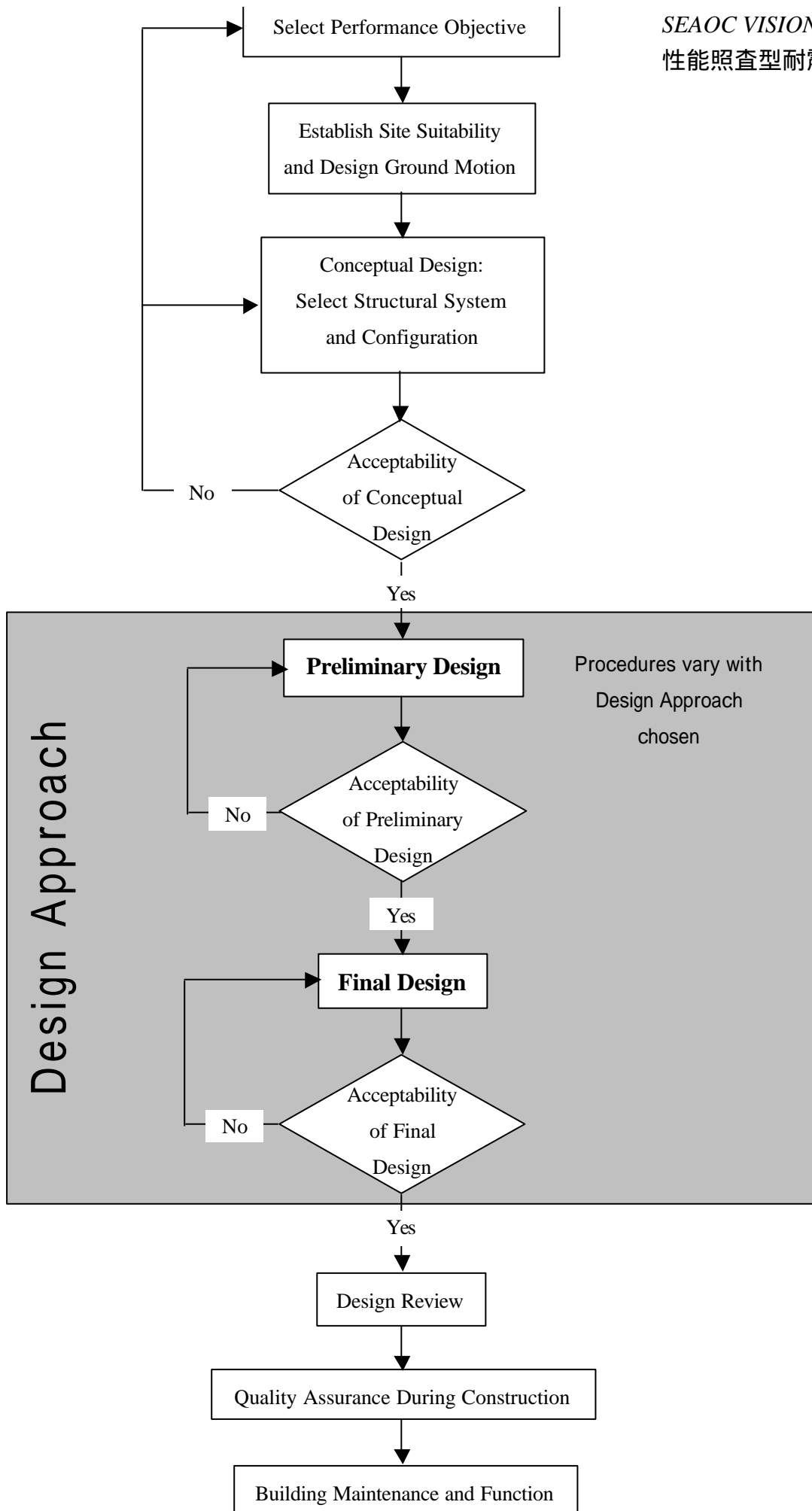
Fig: Methodology for Performance Based Engineering
